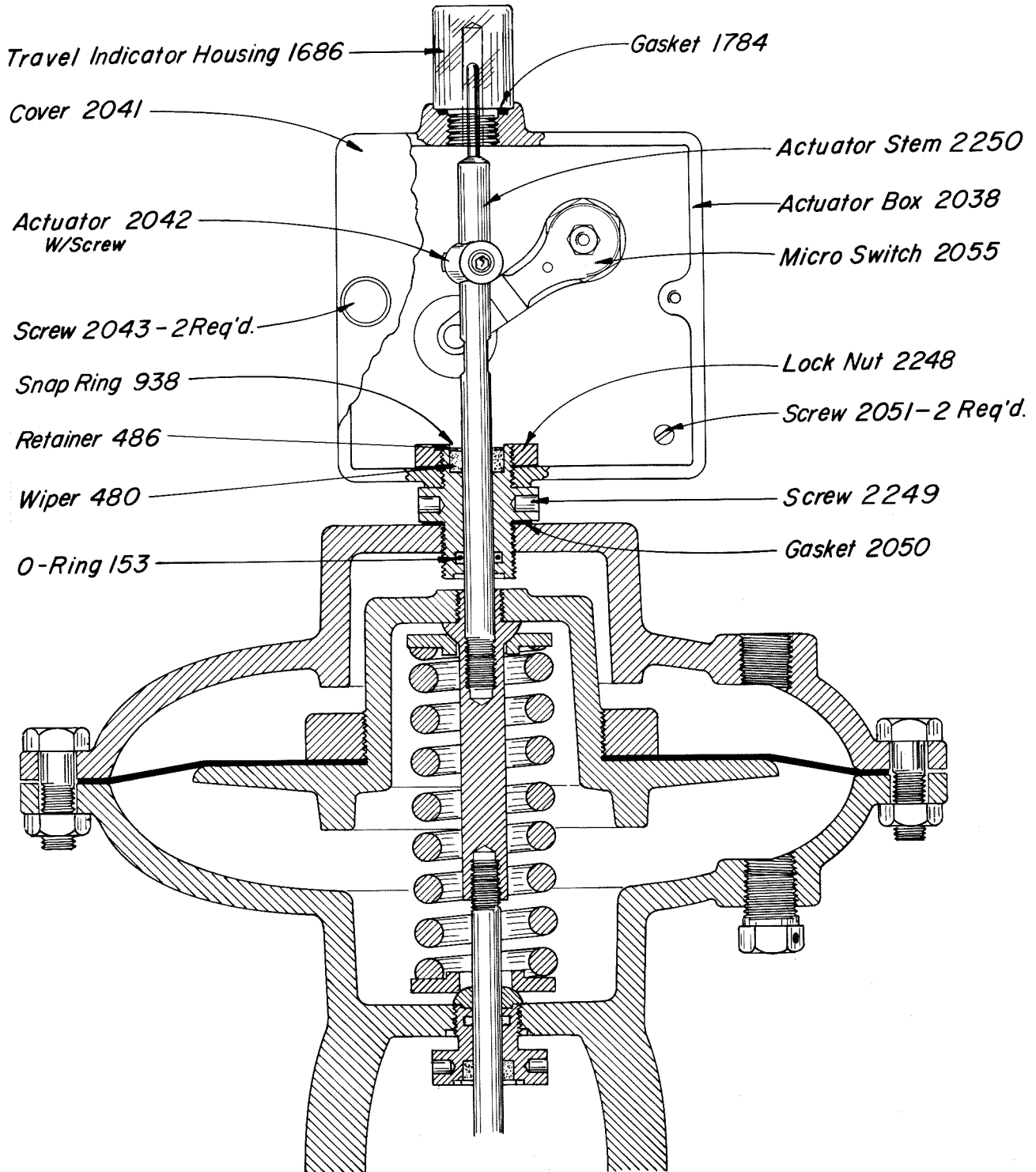
1" & 2" HPMV SMA/T-PO w/MICRO SWITCH
